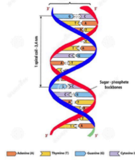
DNA double helix
